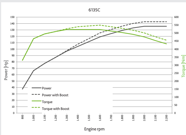
6135 C engine figures.
